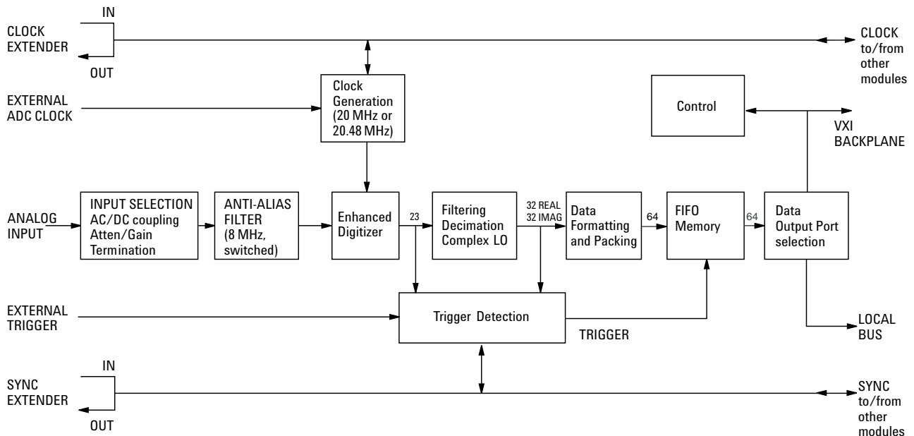
Figure 1: Agilent E1437A Block Diagram
